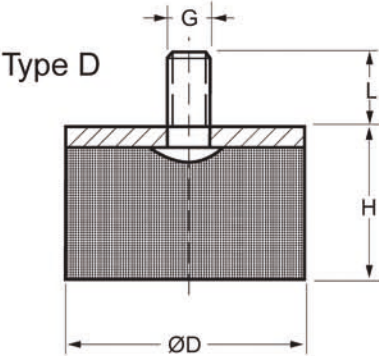
Cylindrical mountings type D
