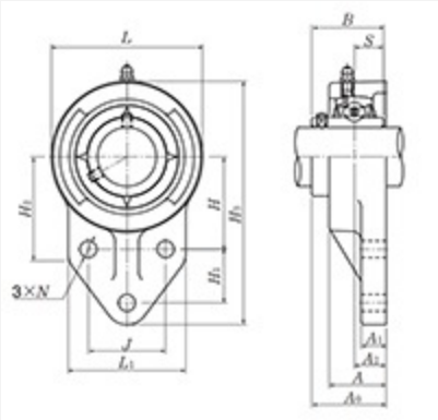
Three Bolt Flanged Unit, Cast Housing, Set Screw, UCFH Type - Dimensions
