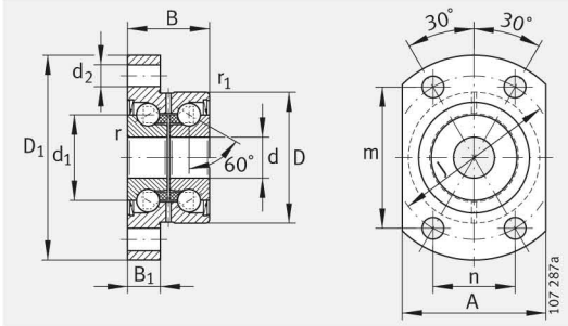
ZKLFA...2RS, ZKLFA...2Z
